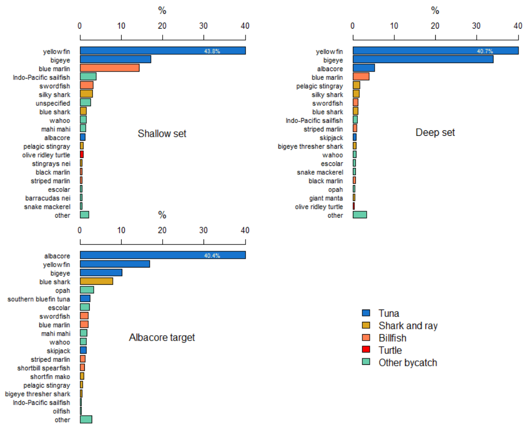
Figure 17: Catch composition of the various categories of longline fisheries operating in the WCPO based on observer data from the last five years' data.
