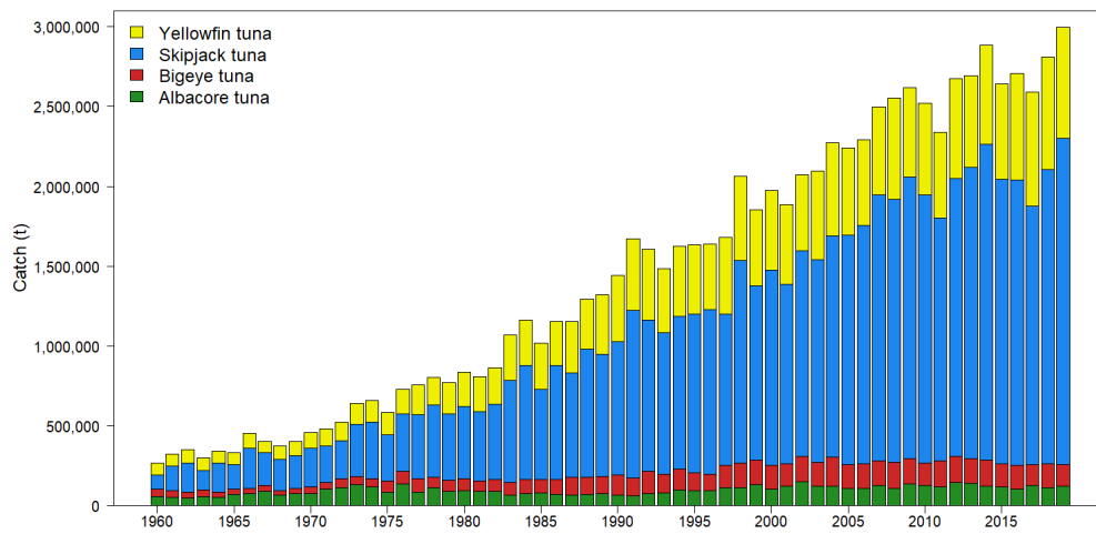
Figure 2: Catch (metric tonnes) by gear (top) and species (bottom) for the western and central Pacific region, 1960–2019. Note: data for 2019 are preliminary.
