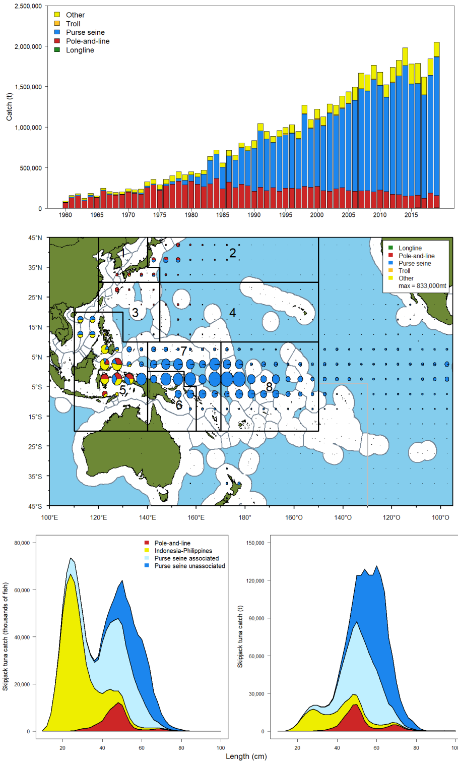
Figure 6: Time series (top), recent (2015–2019) spatial distribution and assessment regions (middle), and size composition (average for last five years) of skipjack tuna catch by gear for the WCPO.
