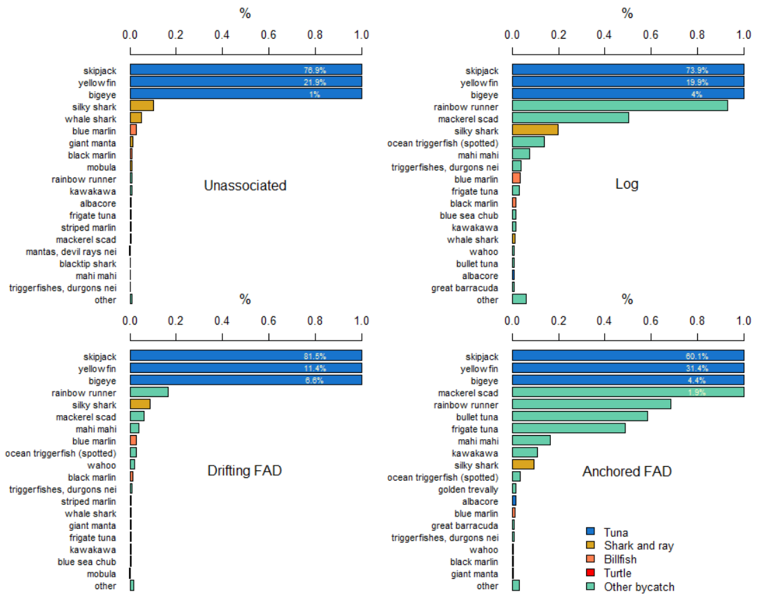
Figure 16: Catch composition of the various categories of purse seine fisheries operating in the WCPO based on observer data from the last five years' data. Note: Species comprising less than 0.01% of the catch are summed in the "other" category.
